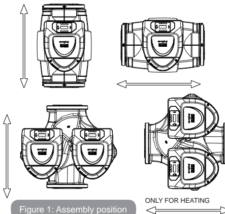
Figure 1: Assembly position
