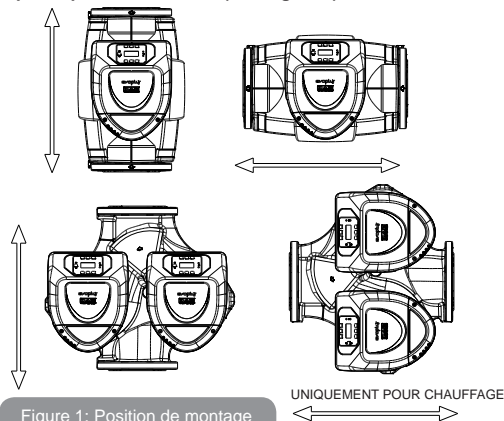
Figure 1: Position de montage
