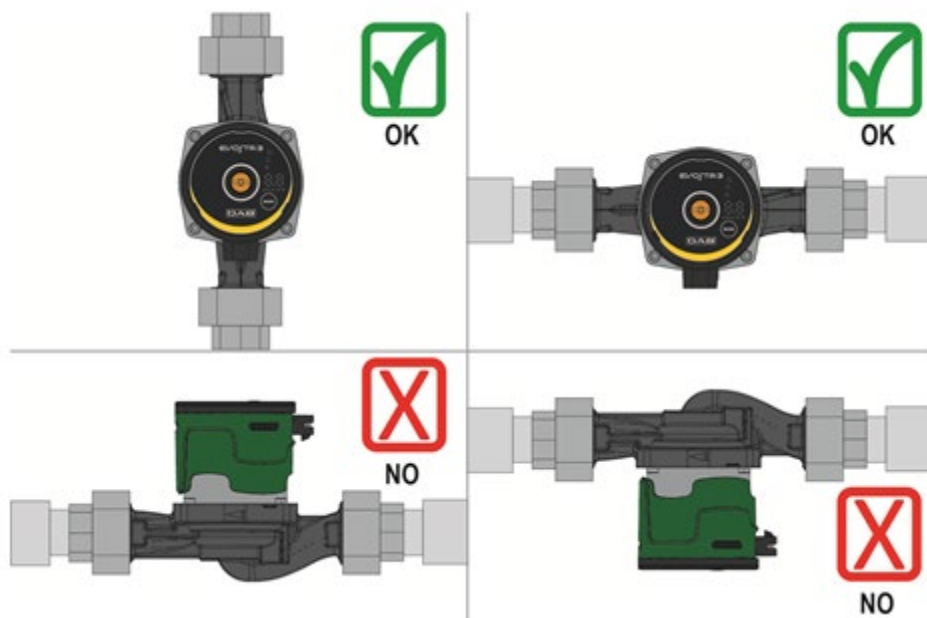
Figure 3: Assembly position
