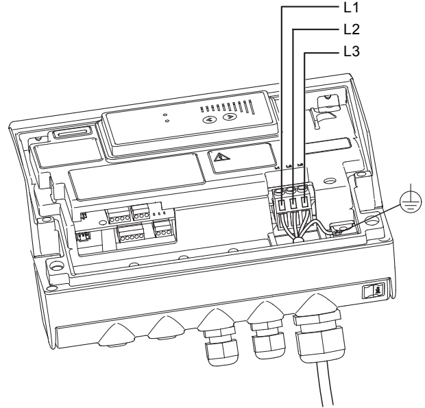
Fig. 3 Mains connection
