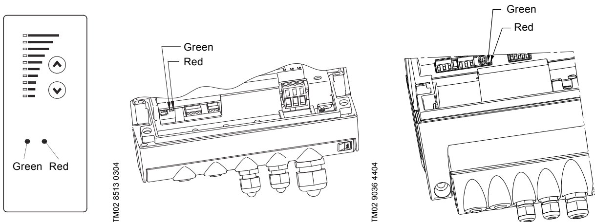
Fig. 33 Position of indicator lights on threeE-phase pumps
